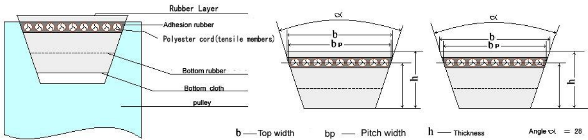
ANGLE CUTTING
