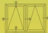
DRAWING/NO. AW80-002 80mm Frame Awning Window layout
