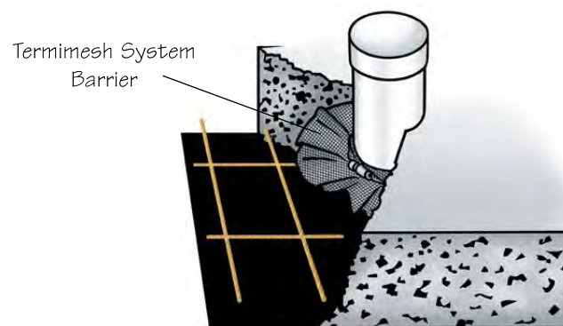
Service Pipe Installation
