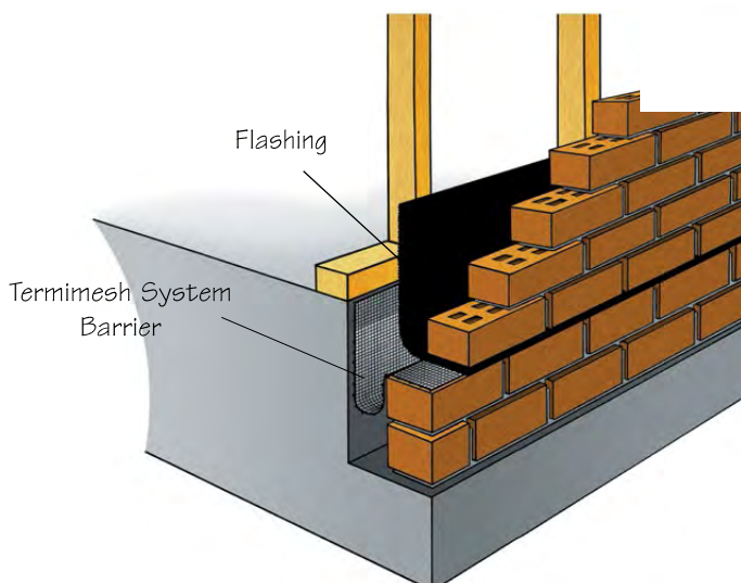
Installation to Stud Wall Construction
