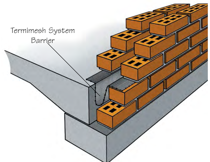
Installation to Double Brick Construction
