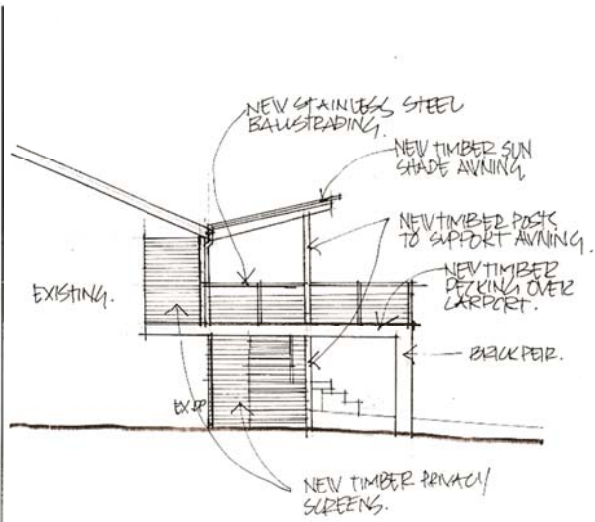
Side Elevation Option A
