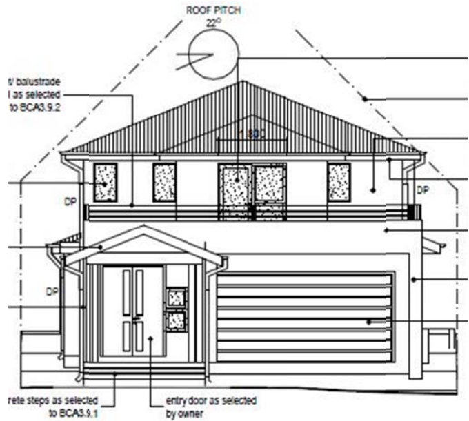
front elevation 1
