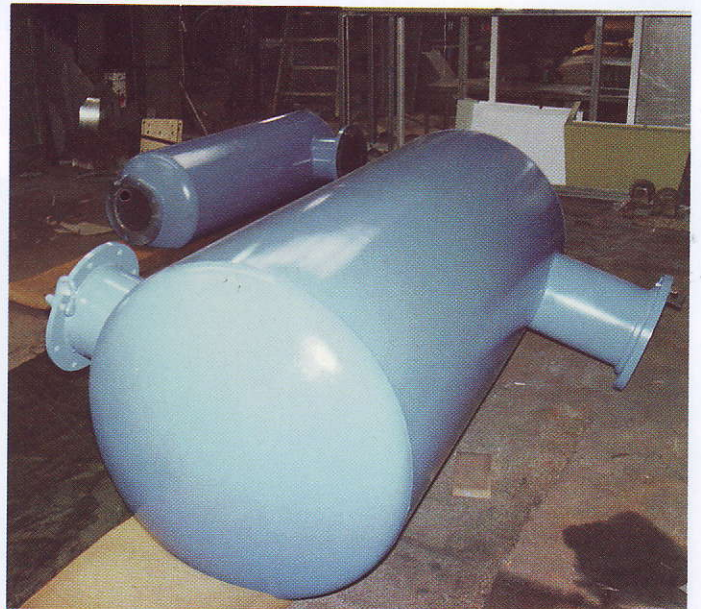
REACTIVE SILENCERS FOR LOW FREQUENCY ATTENUATION
