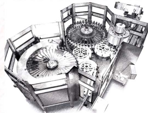
No-tank filler and capper
