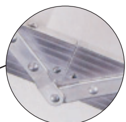
Heavy duty aluminum hinges at rail joints prevent side to side motion
