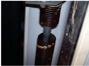
Broken Spring
