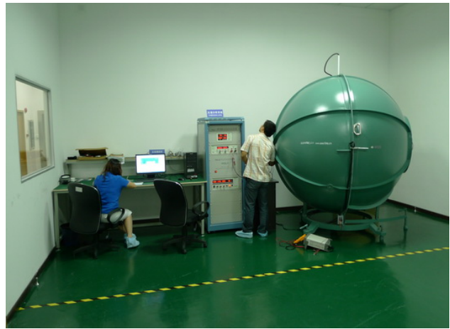
Integrating Sphere with Goniphotometer System
