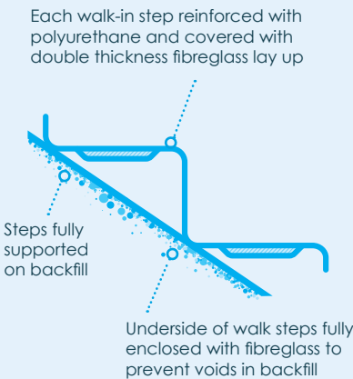
STEP REINFORCEMENT
