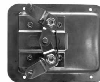
10411 or 10412 Paddle Handle Stainless Steel Handle; Lockable or Non-locking; Multi-point; Size: 108mm x 139.50mm
