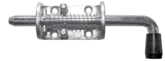
D12-A Zinc plated Steel; 12mm dia. Pin; Dimensions: 74mm x 40mm; Suitable for Left Hand or Right Hand application
