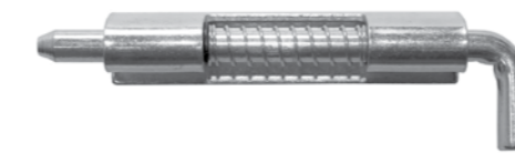
RTH-00004 Zinc plated steel; 6.35mm dia. Pin; Dimensions: 70mm x 14.7mm
