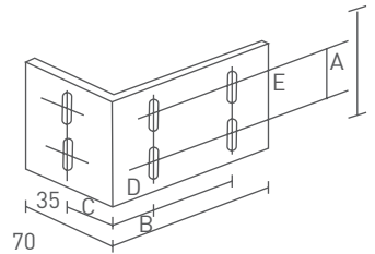
General Purpose Brackets - Long Leg GPBLL Series
