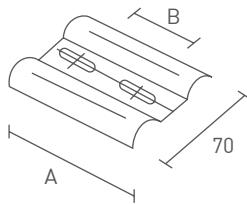
Clamp Plates BUP Series
