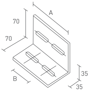
General Purpose Brackets GPB Series
