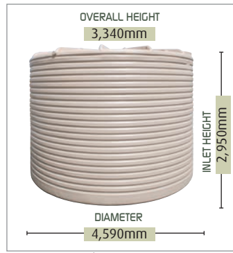
46,800 L | CT10000
