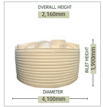
23,600 L | CT5200SQ
