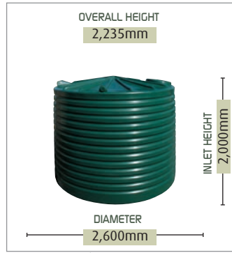
10,000 L | CT2200
