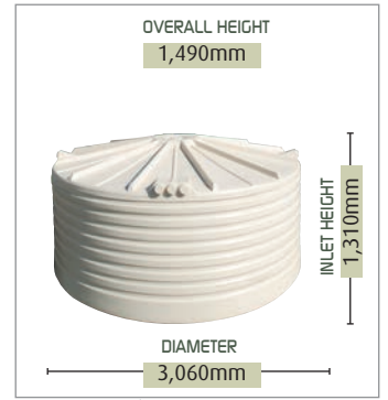
9,500 L | CT2100SQ
