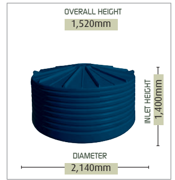
4,500 L | CT1000SQ
