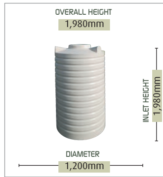
2,000 L | CT440
