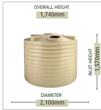
5,000 L | CT1100SQ
