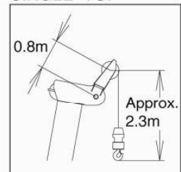
SINGLE TOP
