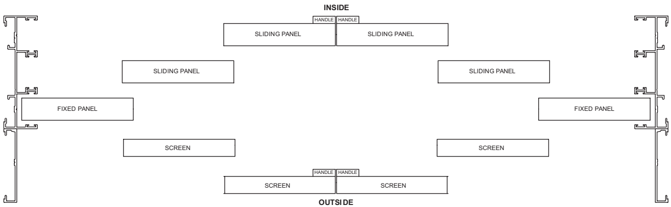
OXXXXO SLIDING DOOR WITH SCREENS FITTED (PLAN VIEW, PANEL LAYOUT ONLY)
