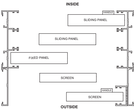
OXX SLIDING DOOR WITH SCREENS FITTED (PLAN VIEW, PANEL LAYOUT ONLY)
