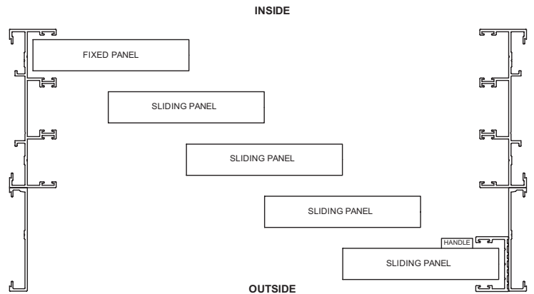
OXXXX SLIDING DOOR (PLAN VIEW, PANEL LAYOUT ONLY) * NO SCREENING POSSIBLE WITH THIS CONFIGURATION
