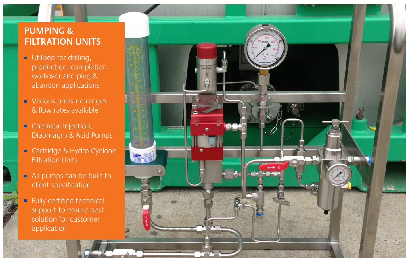
Twin Pod Filtration Unit
